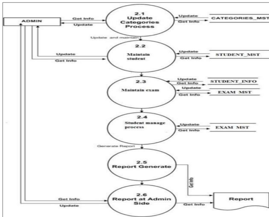
Fig. 4: Data flow diagram Level 2
