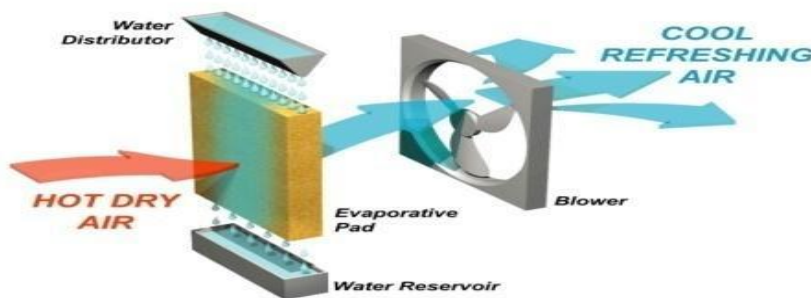
Fig. The basic principle of evaporative cooling
